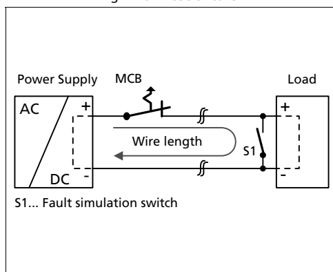
Fig. 22-3 Test circuit
