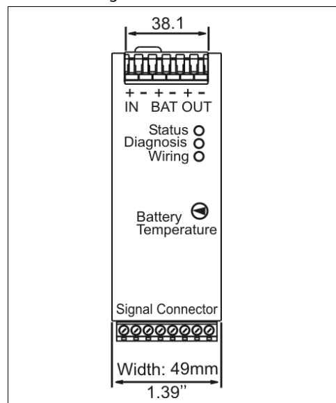
Fig. 25-2 Front view
