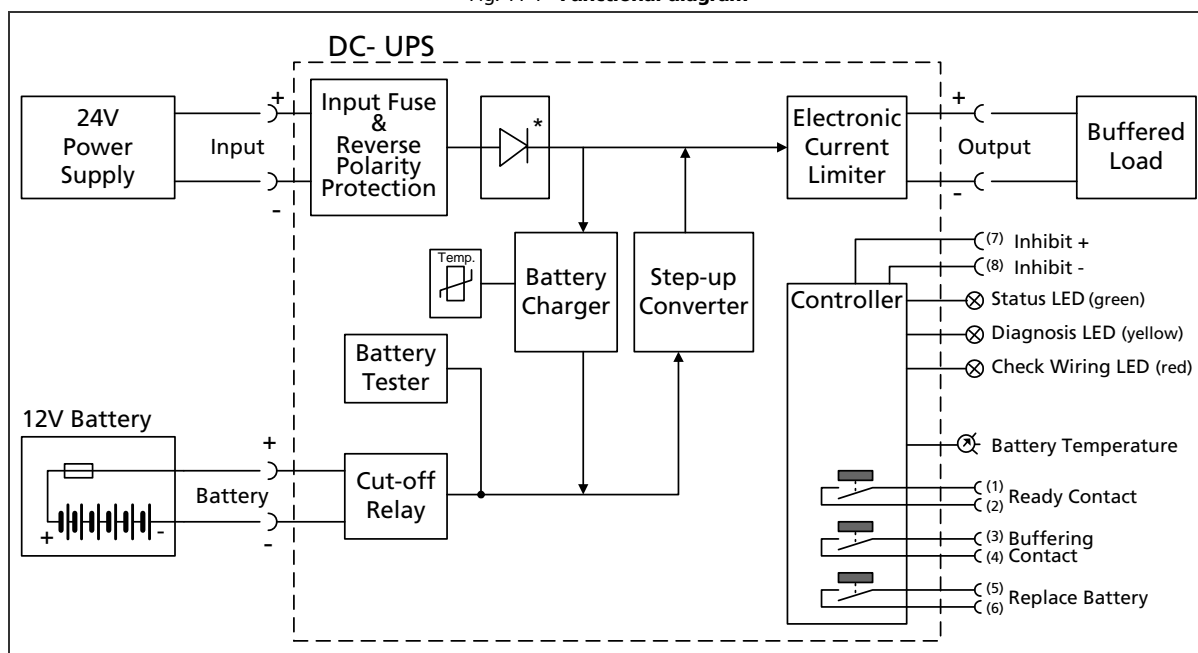
Fig. 11-1 Functional diagram
