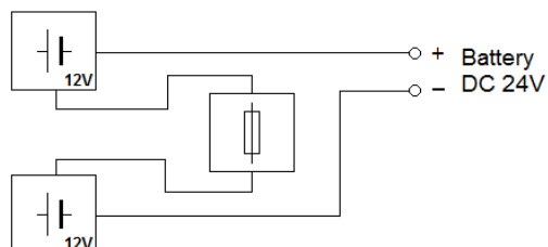
Electrical Diagram
