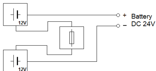
Electrical Diagram
